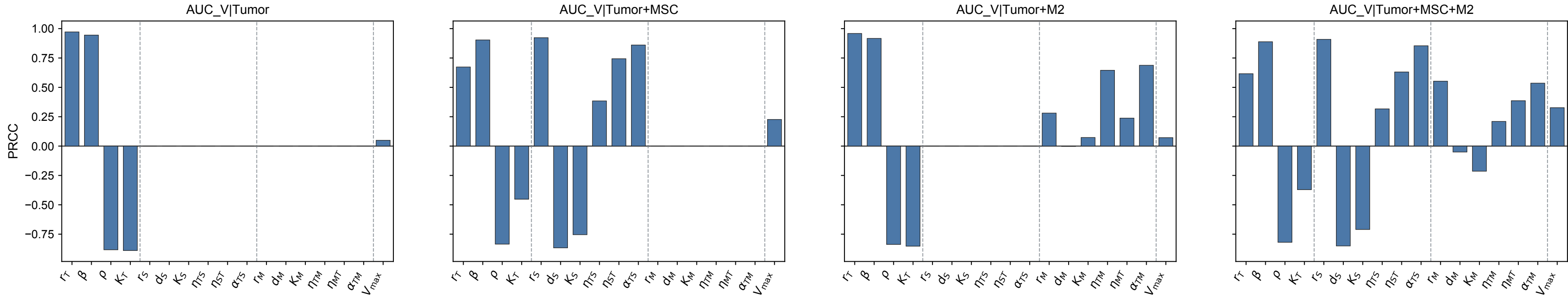
OVCAR3: PRCC on AUC of LP-9 void area V(t)
